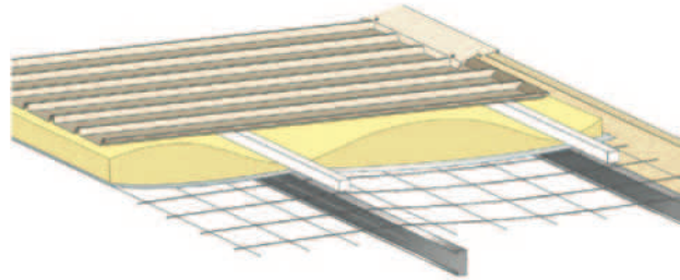
Thermodeck™ spacer.
